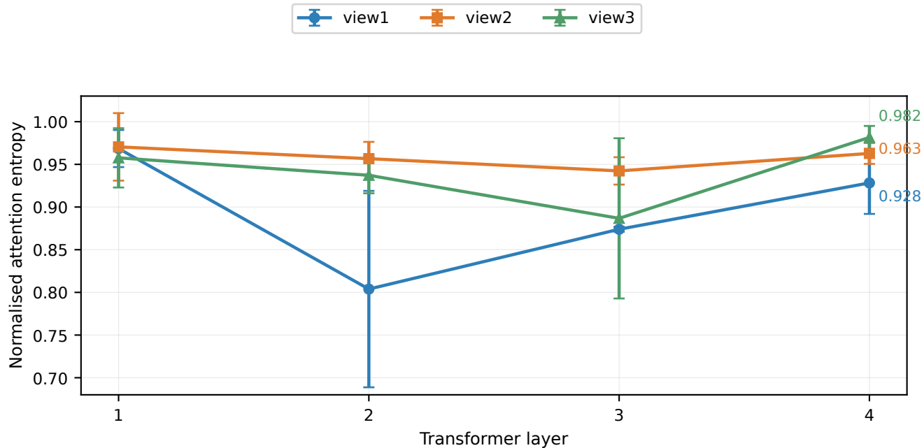
UNSW-NB15 attention concentration by depth (mean \pm std over seeds 42, 123, 456)
