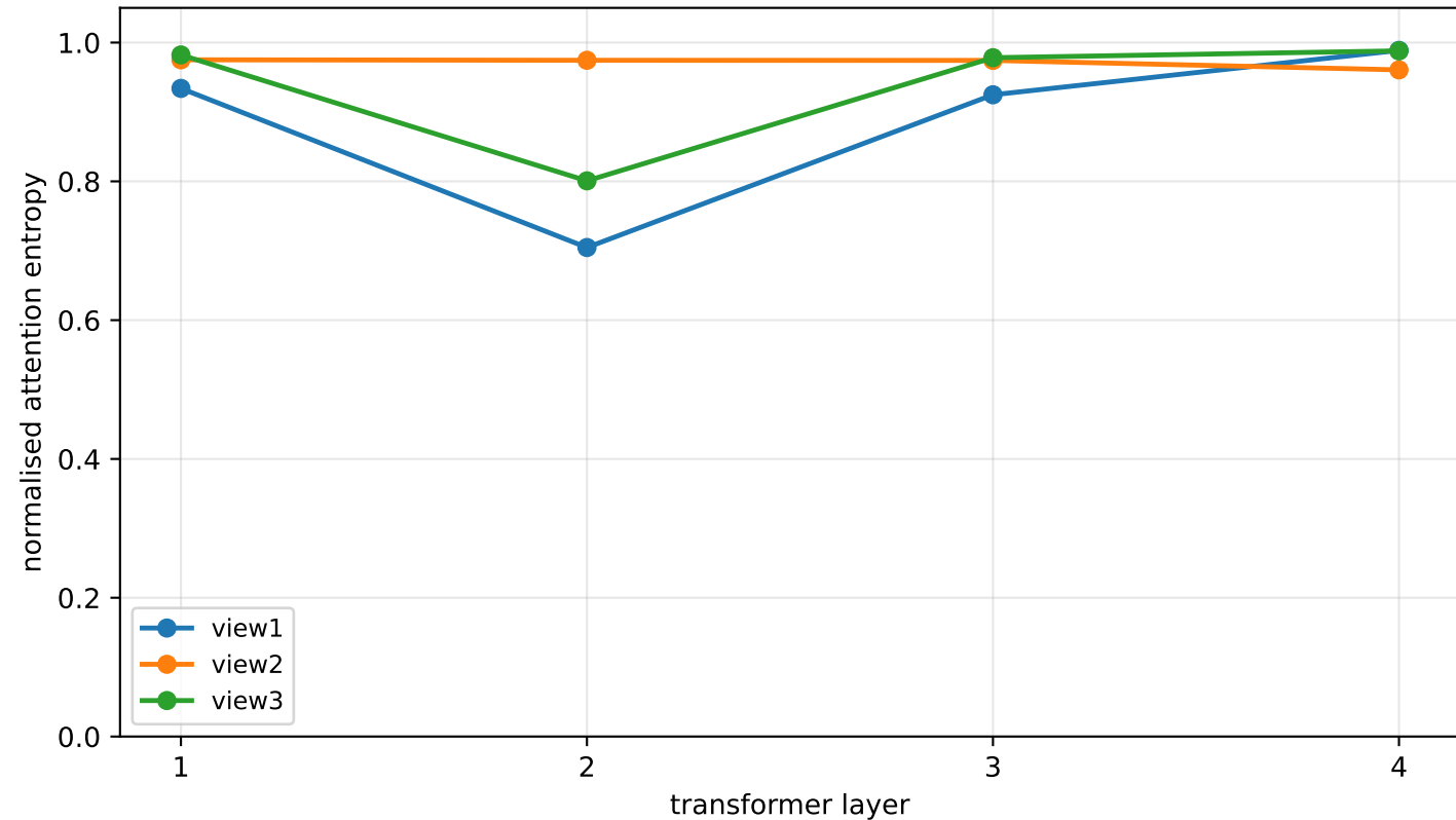
UNSW-NB15 - attention concentration by depth, seed 123 1.0 is uniform across features; lower means the view has specialised
