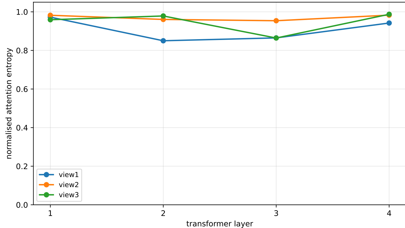
UNSW-NB15 - attention concentration by depth, seed 456 1.0 is uniform across features; lower means the view has specialised
