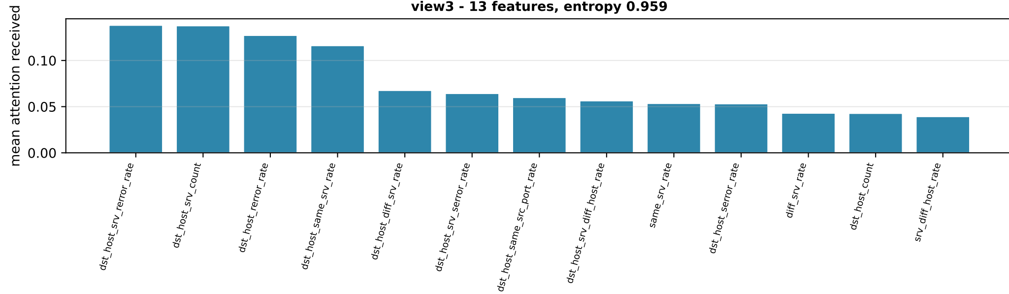
view3 - 13 features, entropy 0.959
