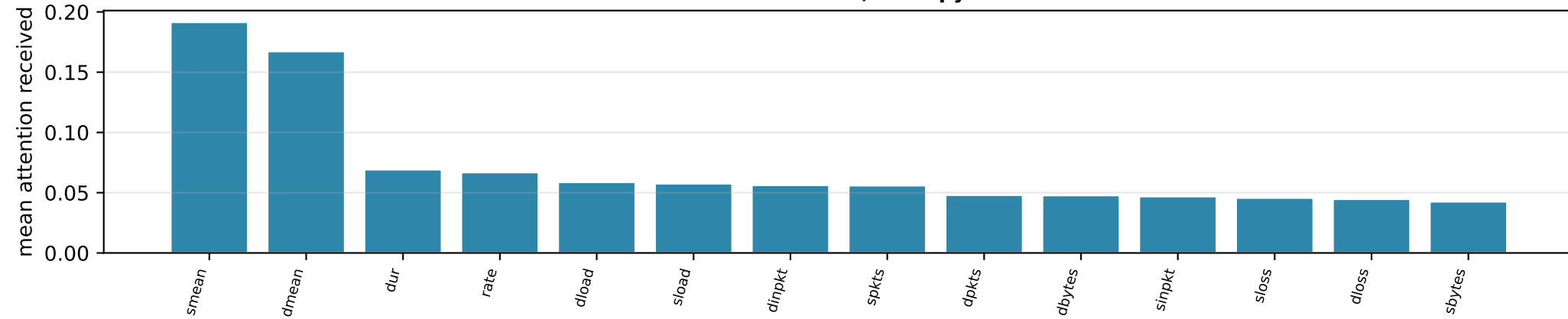
view1 - 14 features, entropy 0.942
