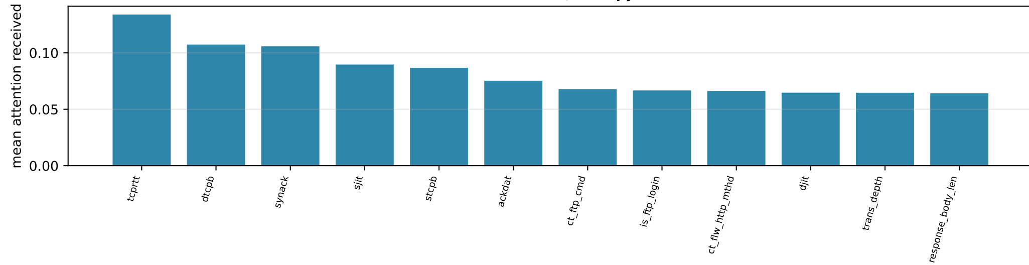
view3 - 12 features, entropy 0.987
