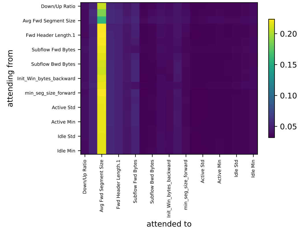
view3 (21 features) entropy 0.941
