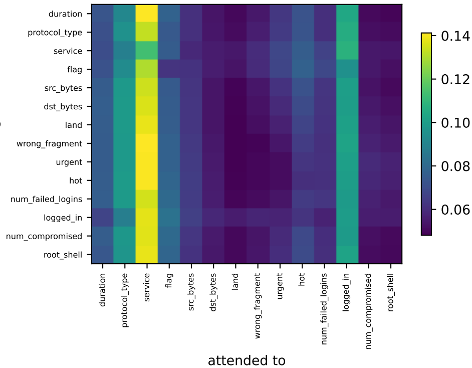
view1 (14 features) entropy 0.982
