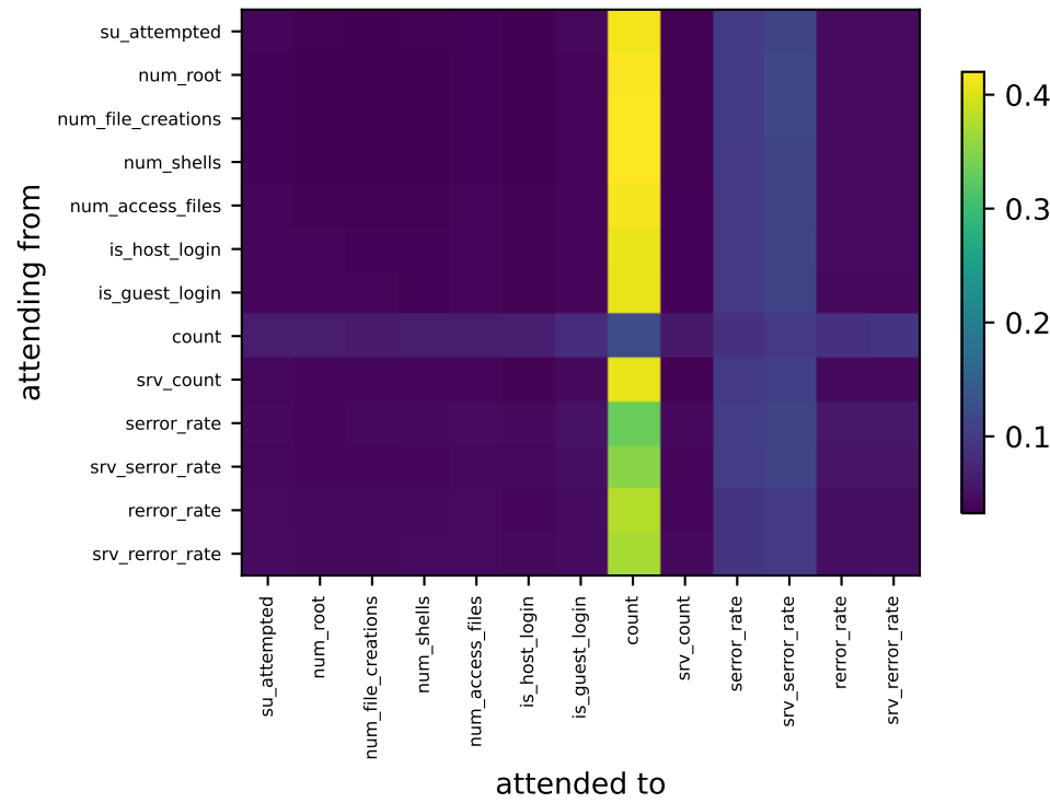
view2 (13 features) entropy 0.844
