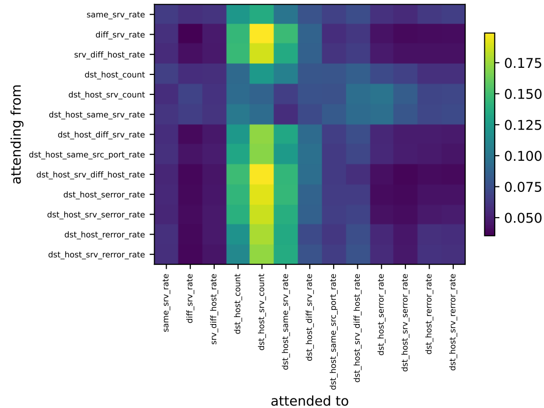
view3 (13 features) entropy 0.965
