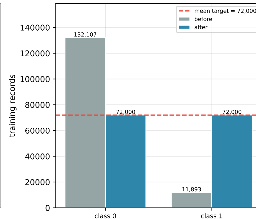
CIC-IDS-2017 (seed 42)
