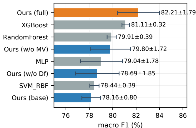
CIC-DDoS2019
