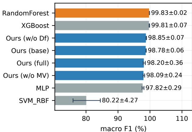
CIC-IDS-2017
