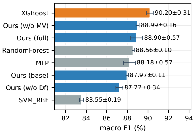
CIC-IDS-2017
