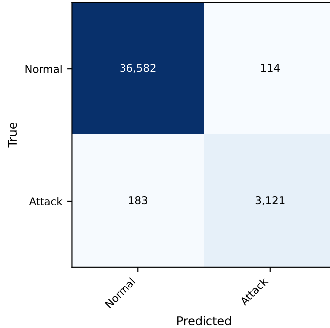
w/o Multi-view
