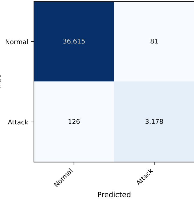
Full Model
