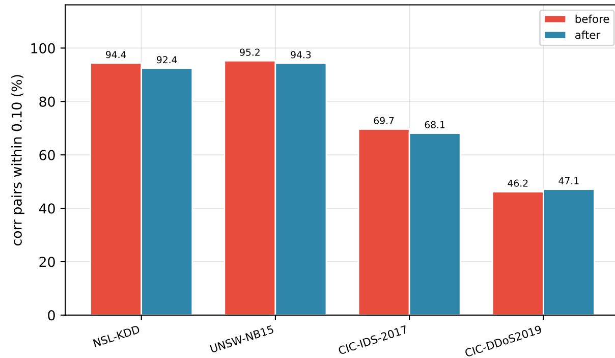
corr pairs within 0.10 (%) (higher is better)
