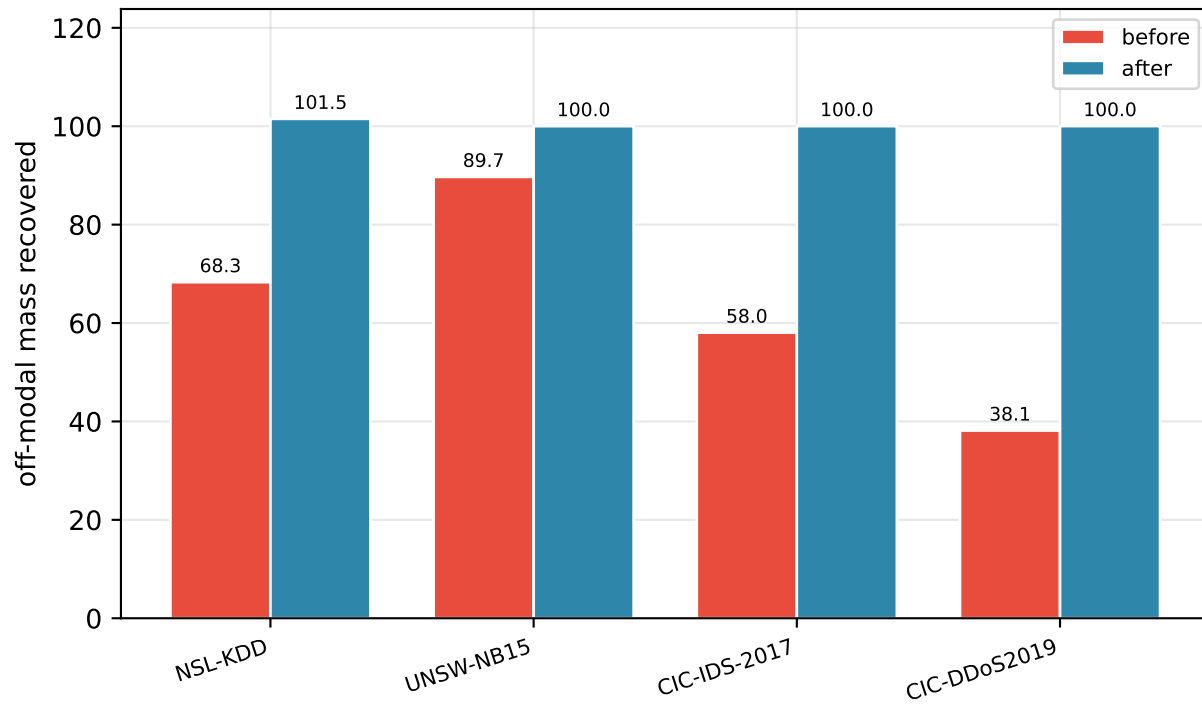
off-modal mass recovered (higher is better)
