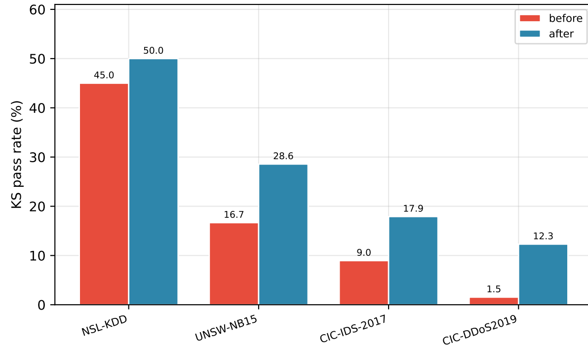
KS pass rate (%) (higher is better)
