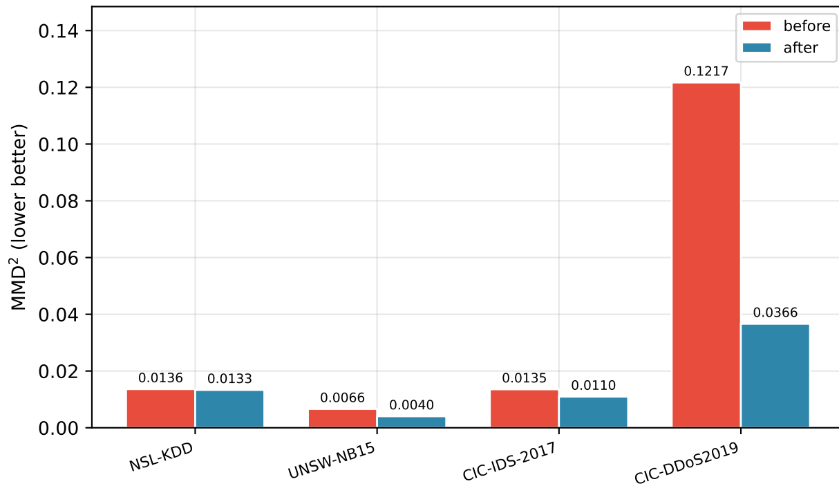
MMD 2 (lower better) (lower is better)
