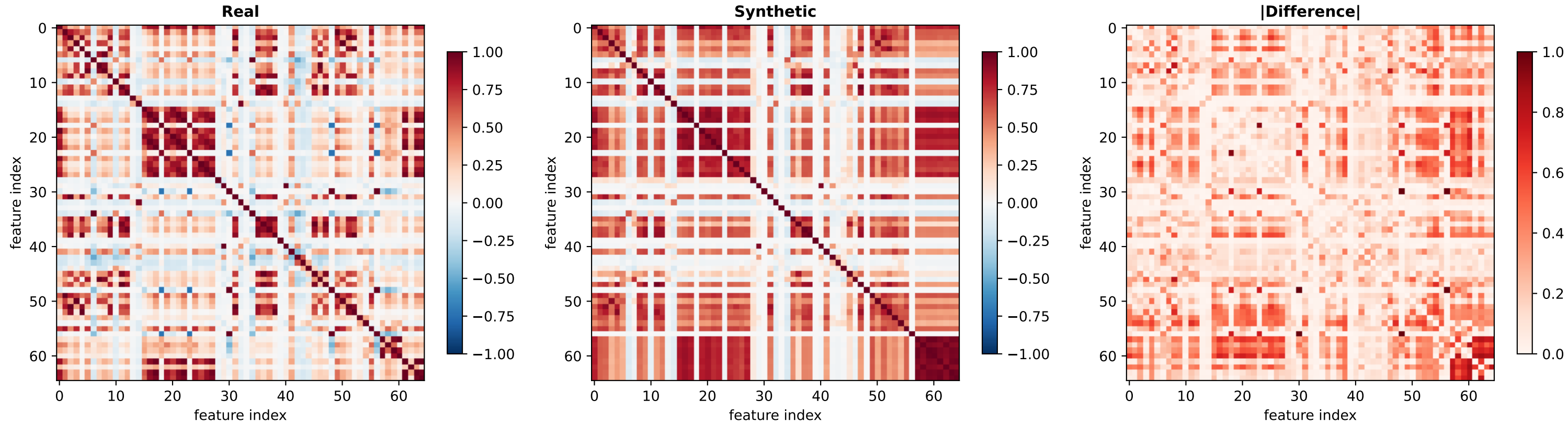
CIC-DDoS2019 - Correlation Structure (seed 123) \text{mean}|d|=0.179 within 0.10: 46.2%
