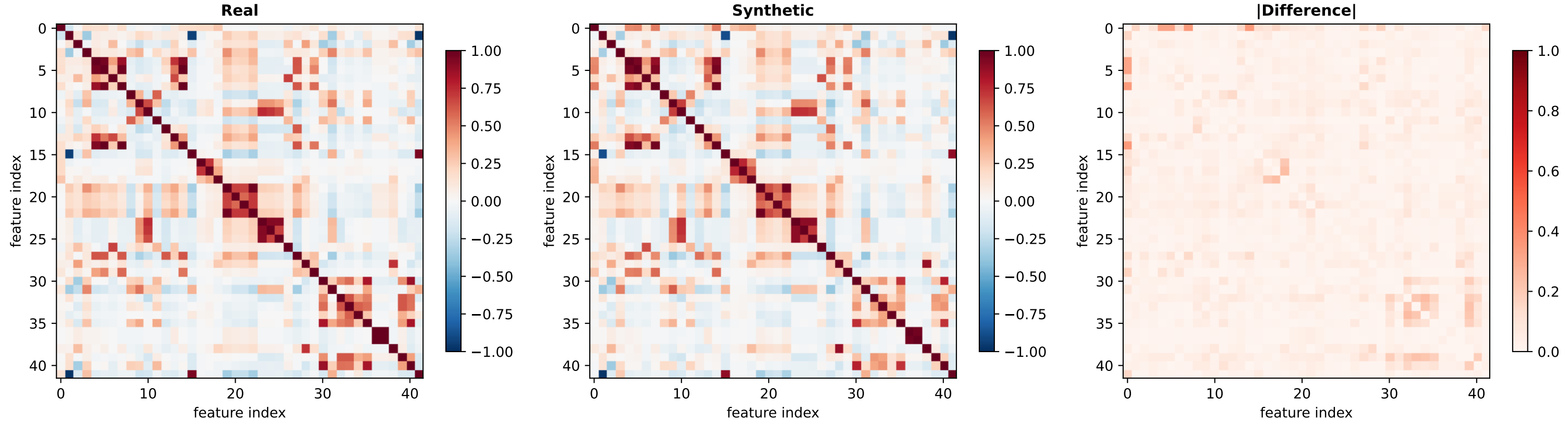
UNSW-NB15 - Correlation Structure (seed 123) mean|d|=0.030 within 0.10: 95.2%
