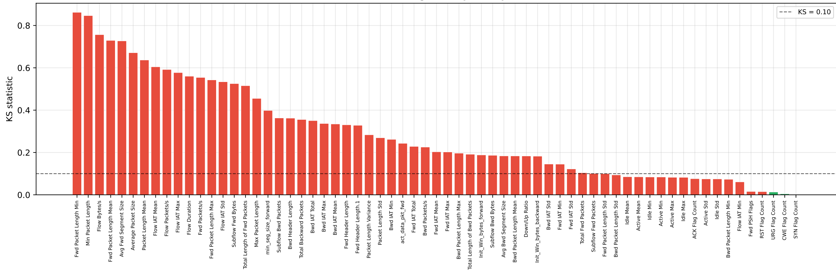
CIC-DDoS2019 - Per-feature KS (green = passes p > 0.05 : 3/65) seed 123
