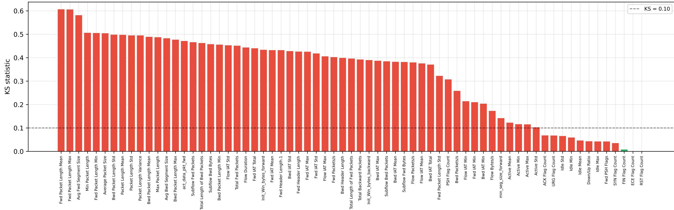
CIC-IDS-2017 - Per-feature KS (green = passes p>0.05 : 3/67) seed 123
