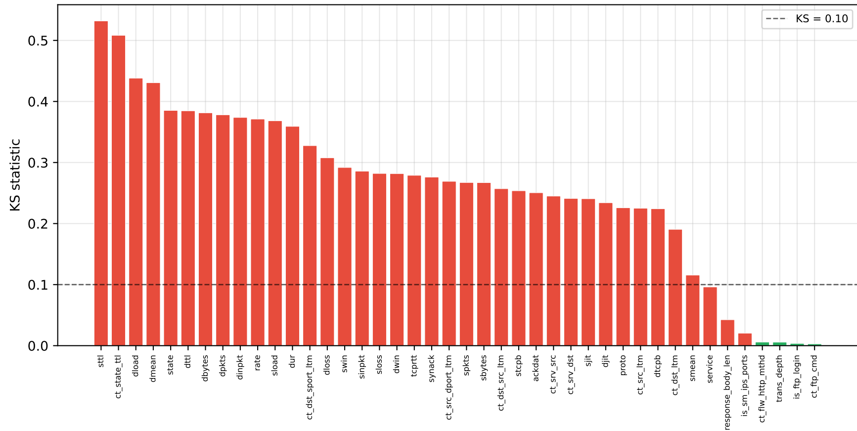
UNSW-NB15 - Per-feature KS (green = passes p > 0.05 : 4/42) seed 123
