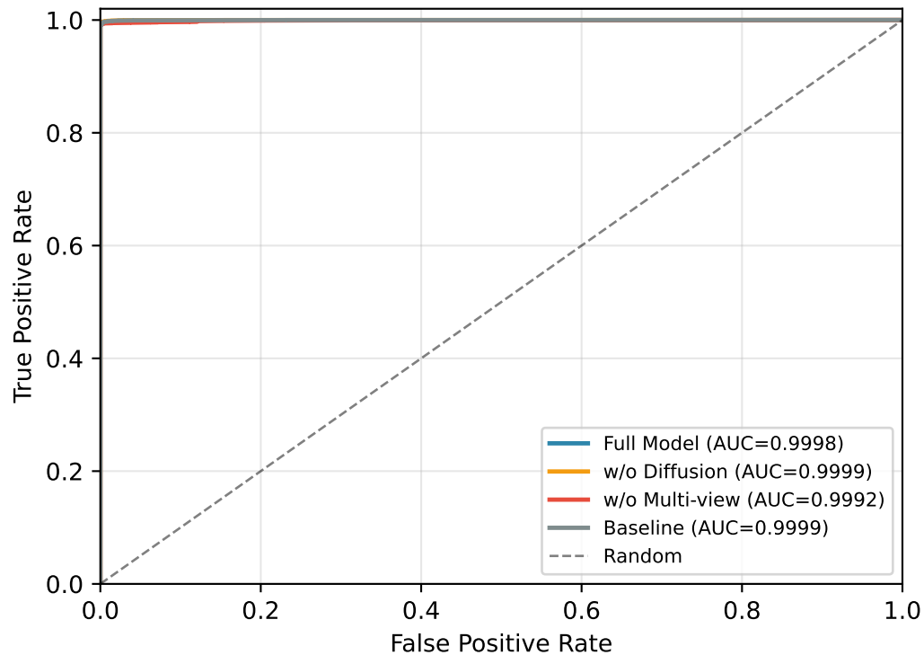
ROC Curve
