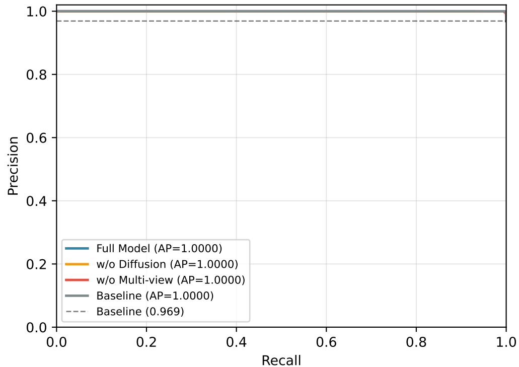
Precision-Recall Curve
