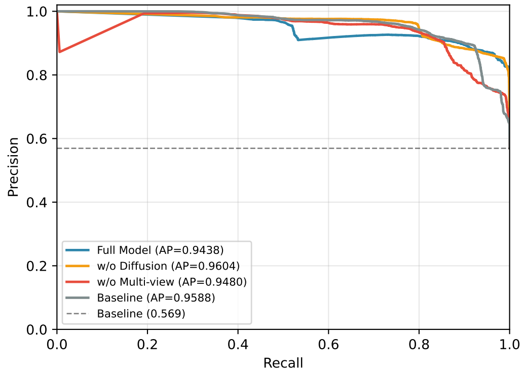
Precision-Recall Curve
