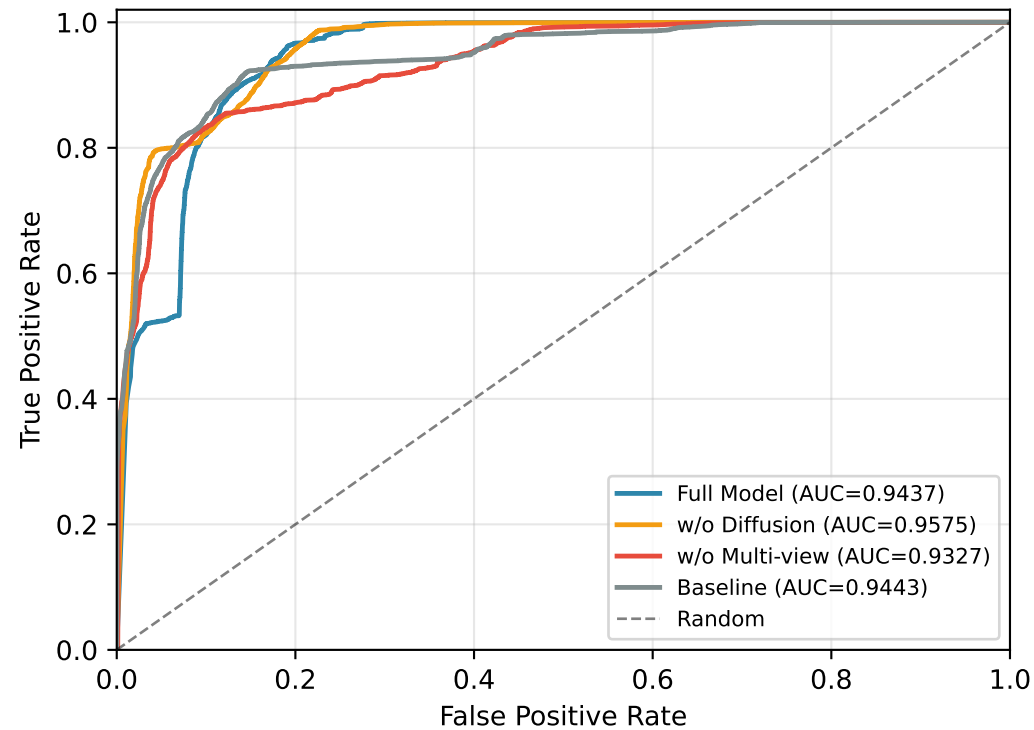
ROC Curve
