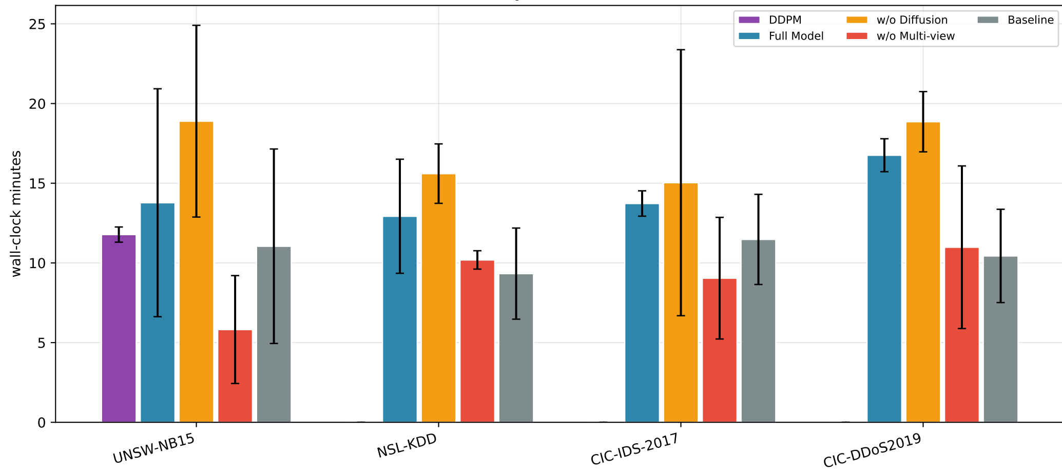
Training cost by stage, mean \pm std over seeds (four datasets ran concurrently, so absolute values include contention)
