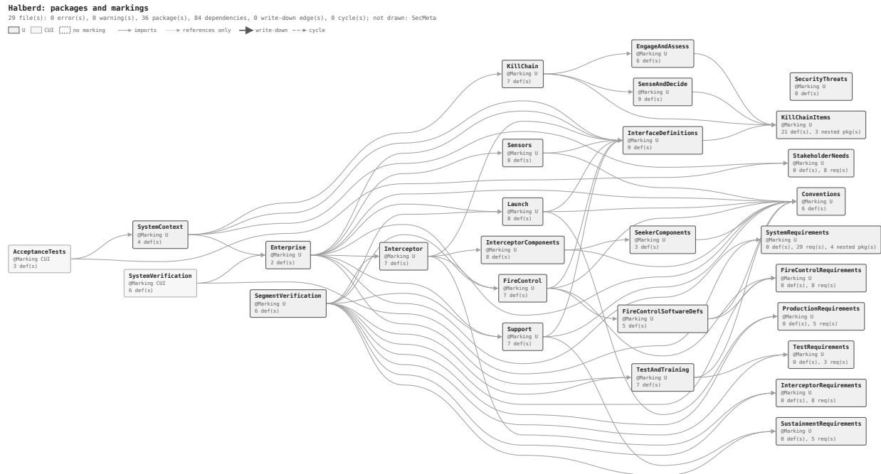
Figure 8: Packages, their dependencies and markings (the SecMeta library hidden). (docs/img/halberd-pkg.svg)
