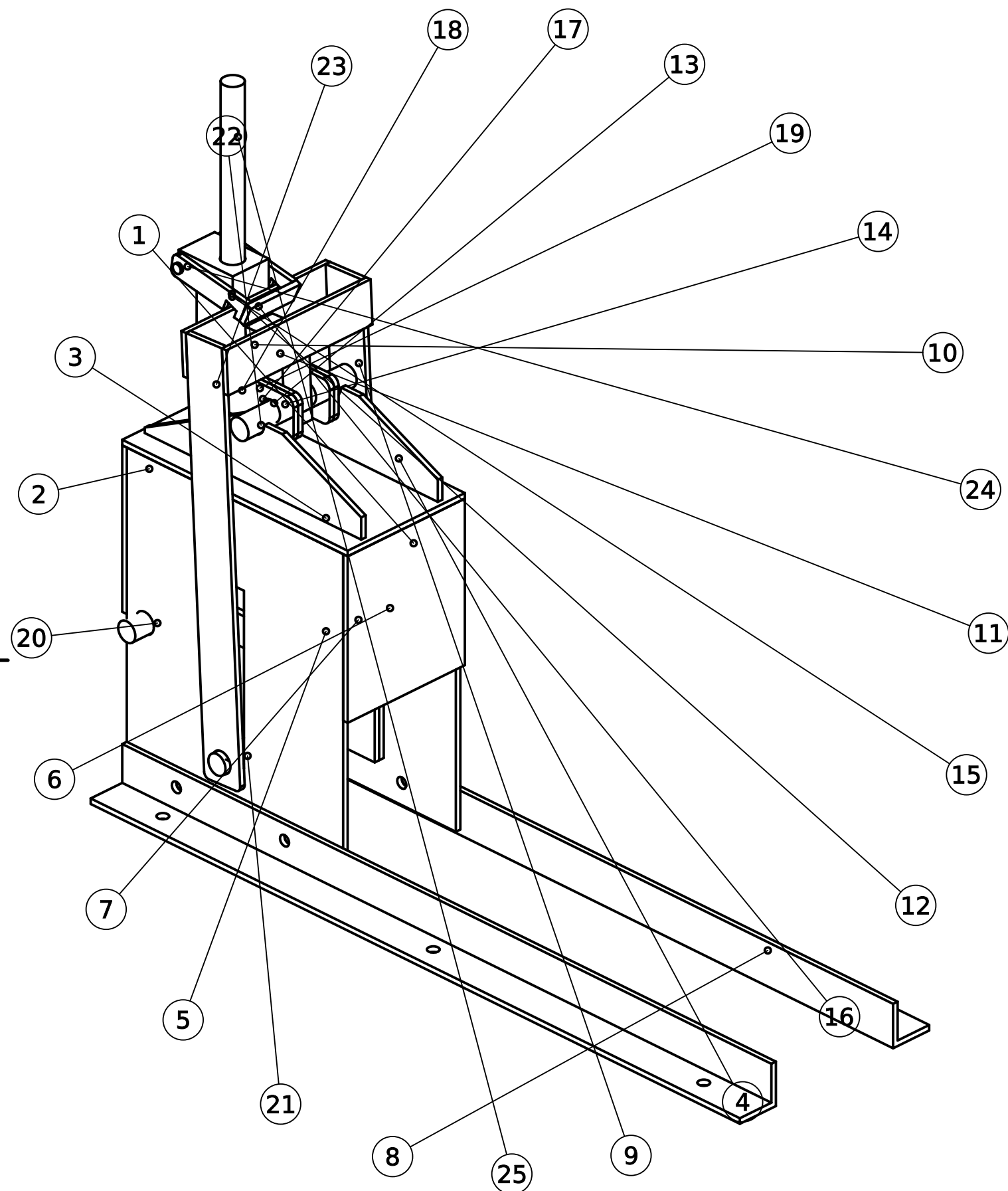
ISOMETRIC VIEW
