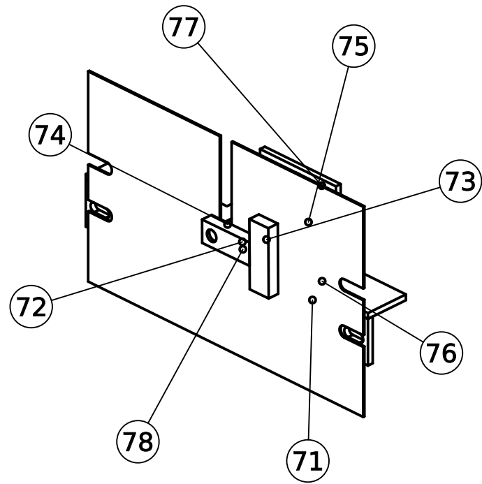
ISOMETRIC VIEW
