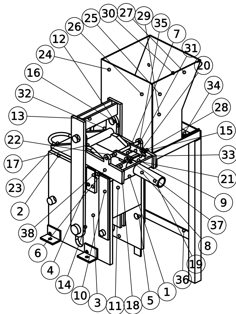
ISOMETRIC VIEW
