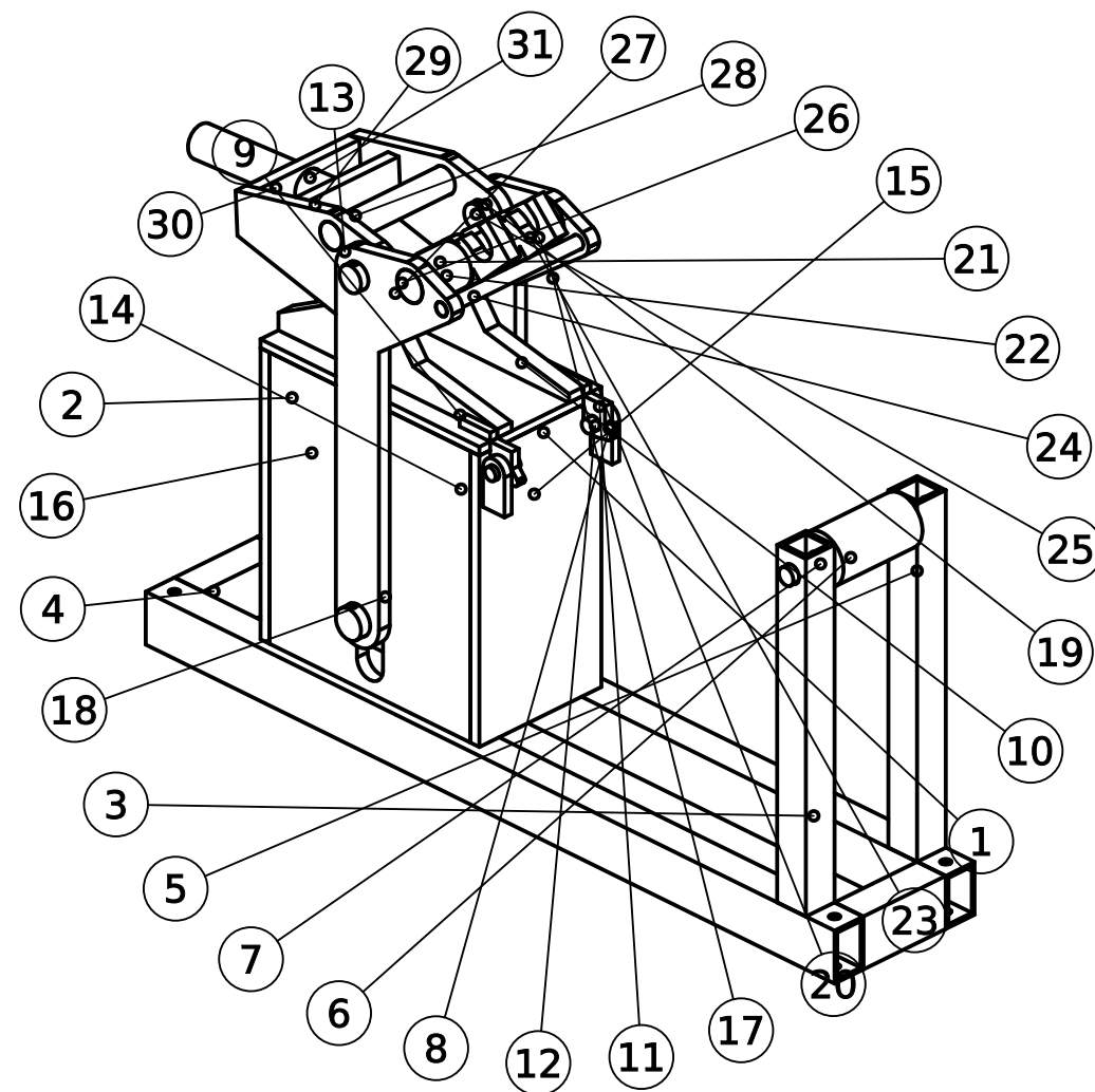
ISOMETRIC VIEW
