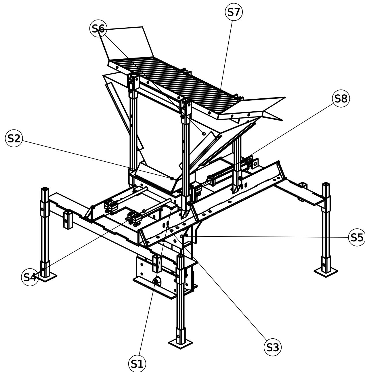
ISOMETRIC VIEW
