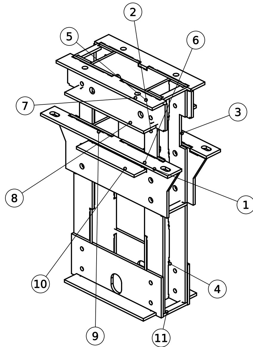
ISOMETRIC VIEW
