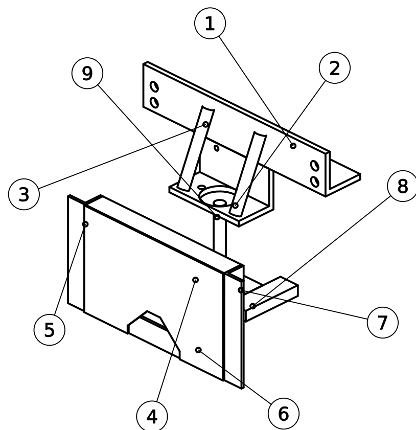
ISOMETRIC VIEW (ARRANGEMENT INDICATIVE)
