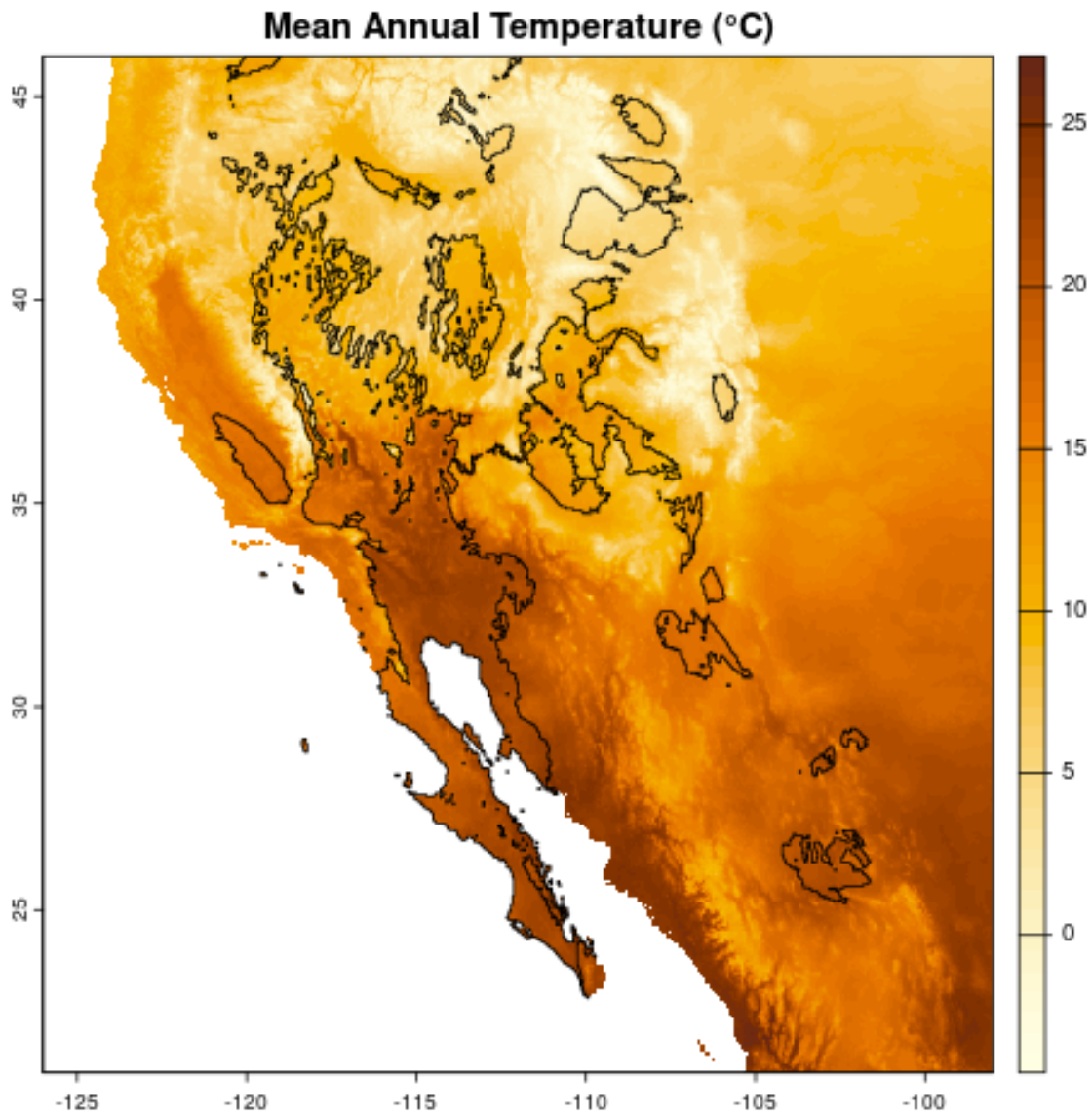
Figure 3: Mean annual temperature of southwestern North America
