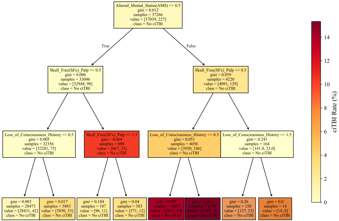
Decision Tree for ciTBI Prediction (max_depth=3)
