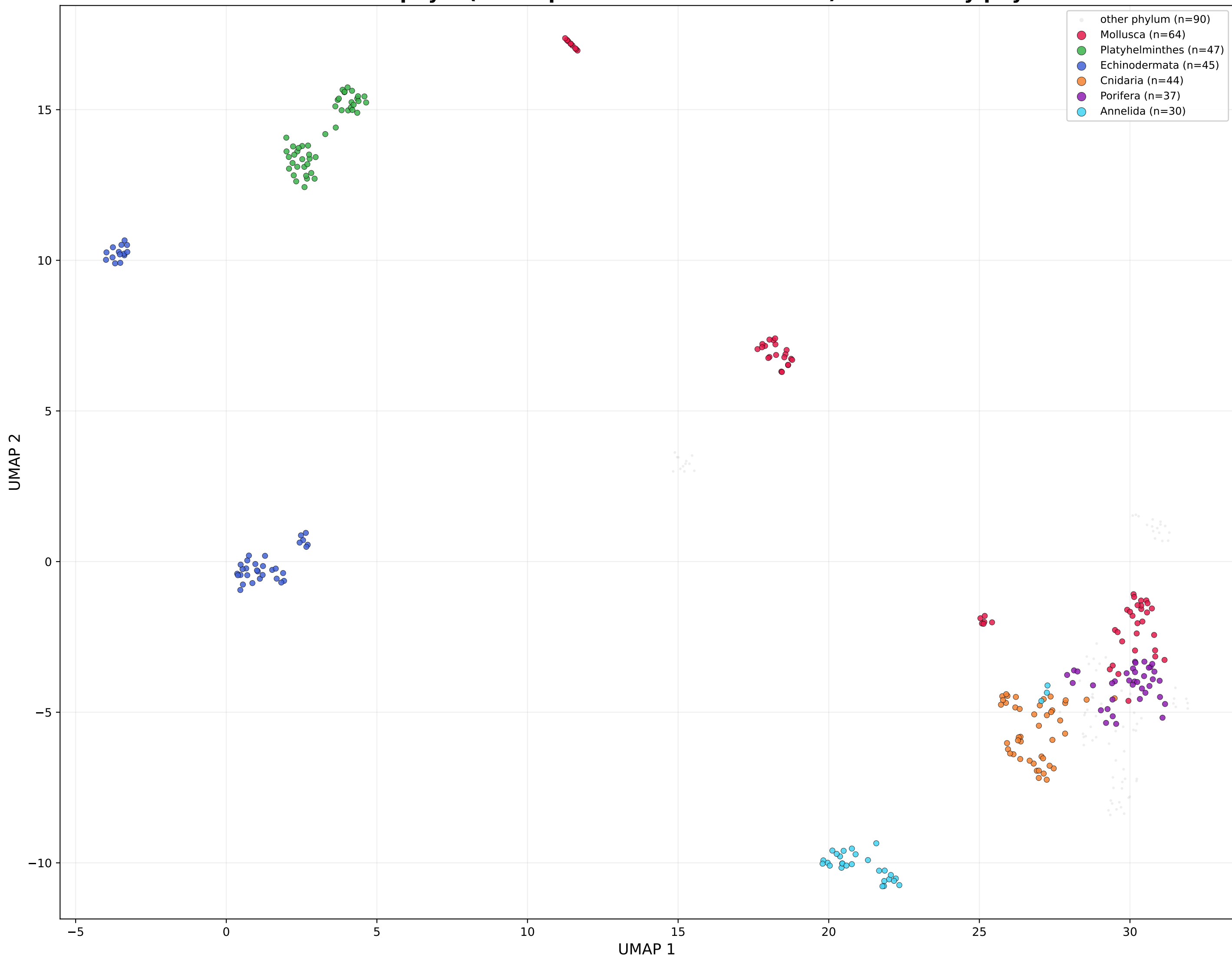
Metazoa minor phyla (Arthropoda+Chordata excluded) — orders by phylum
