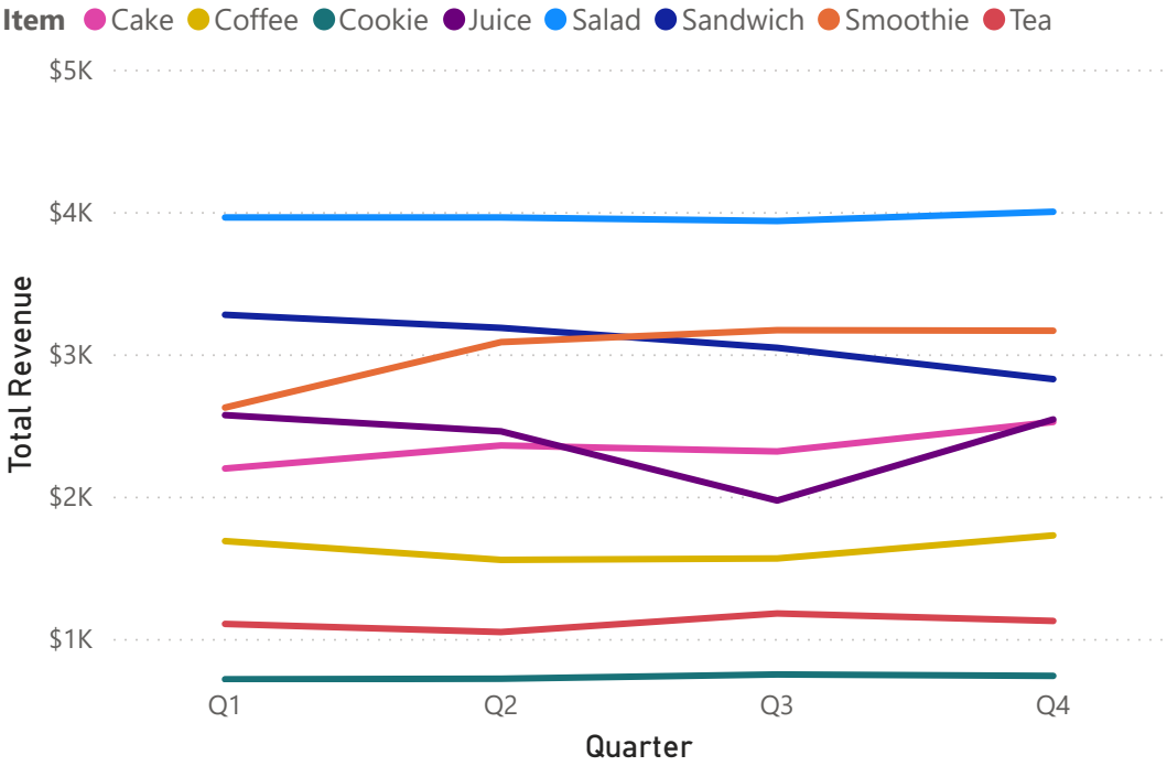
Total Revenue per item
