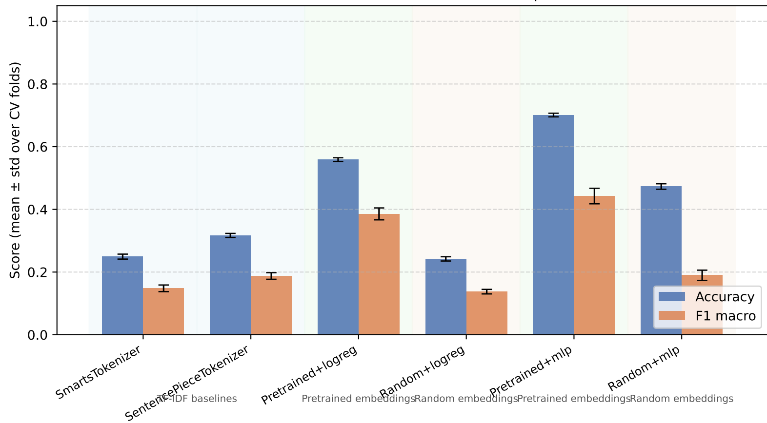
EC Class Classification — Method Comparison
