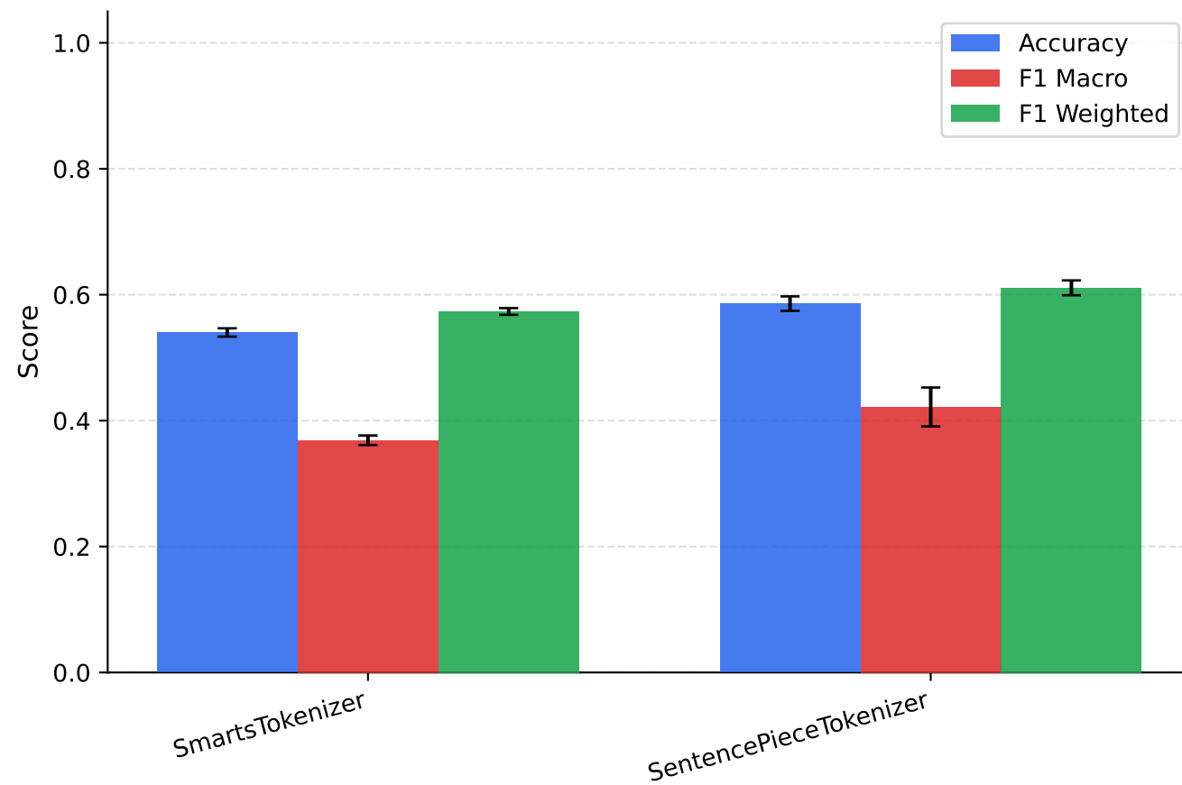
EC Class Classification
