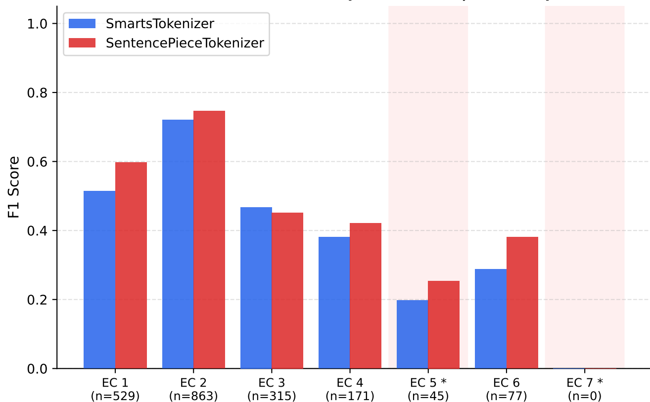
Per-class F1 Score (* rare class, shaded)
