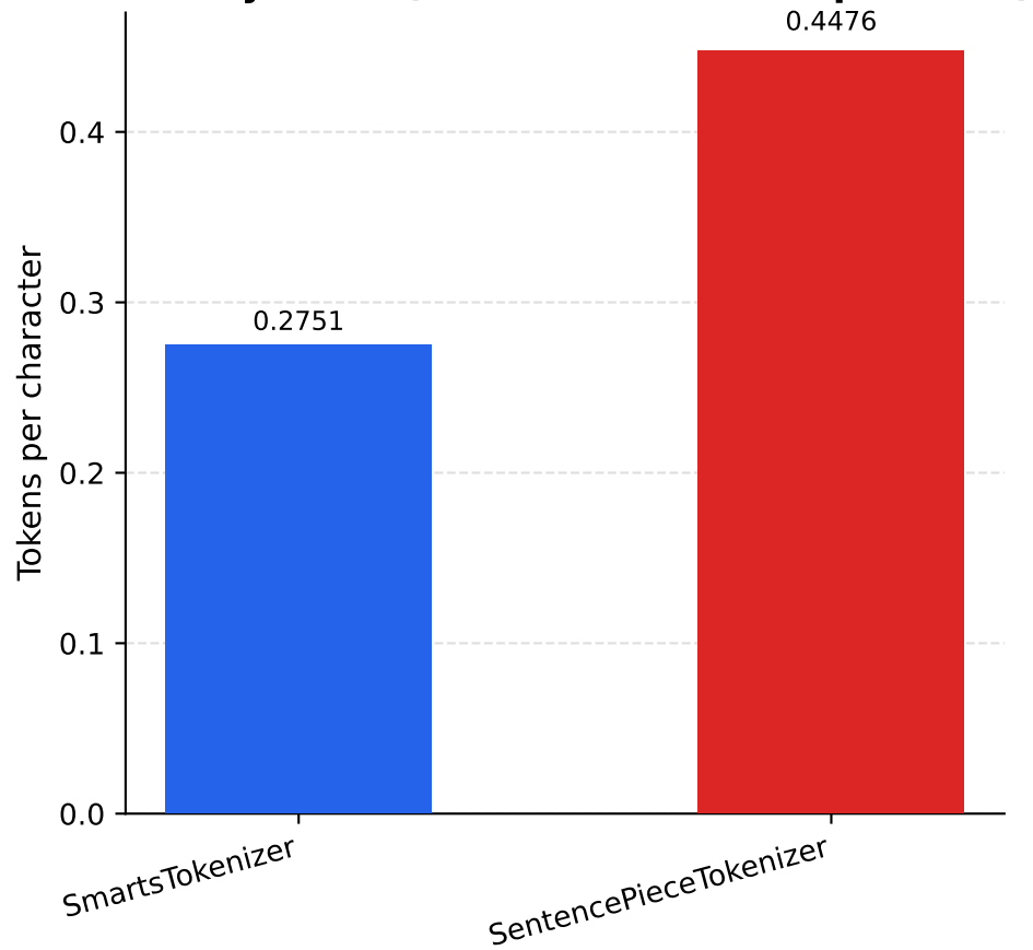
Fertility Ratio (lower = better compression)
