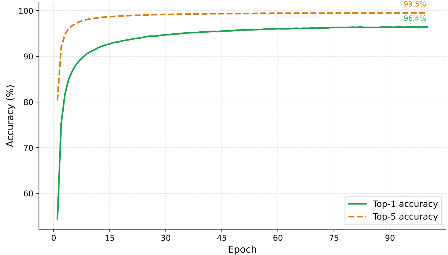
Masked Token Prediction Accuracy
