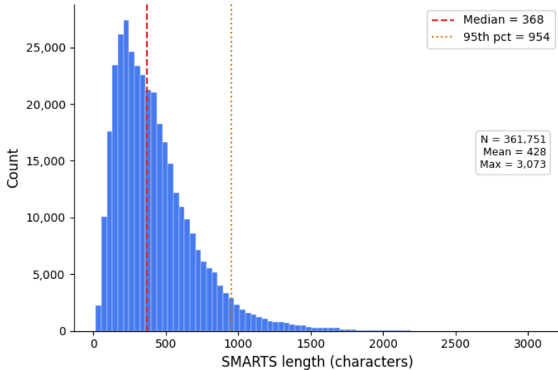
(A) SMARTS Length Distribution
