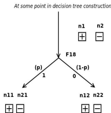
Figure 13: Splitting criterion
