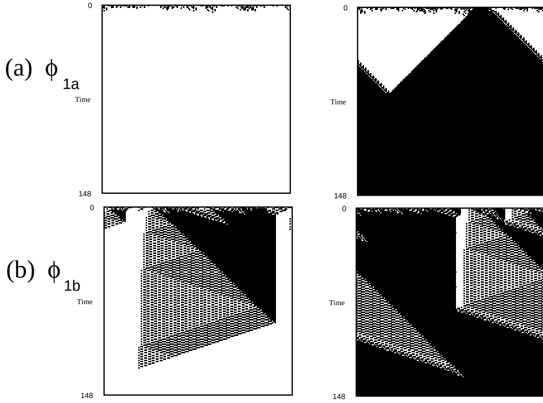
Figure 1: Space-time patterns of four different rules discovered by the GA. The left diagrams have \rho_0 < 1/2 ; the right diagrams have \rho_0 > 1/2 . Fitness increases from (a) to (d). (a) \phi_{1a} . (b) \phi_{1b} . (c) \phi_{1c} . (d) \phi_{1d} . (Continued on next page.)
