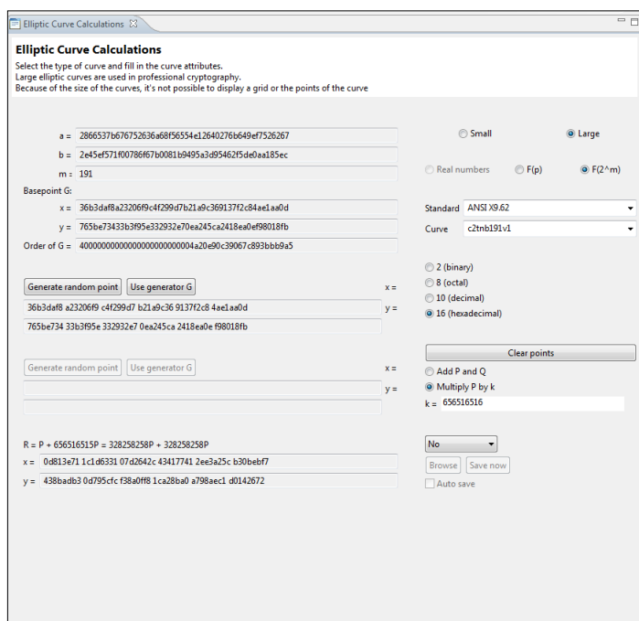
Figure 8: ECC using large numbers
