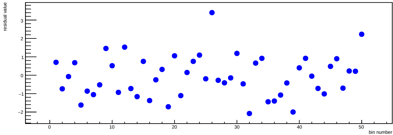
res_hist
