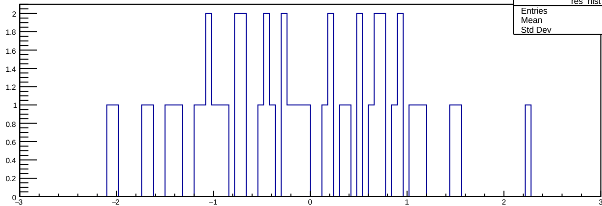
res_hist
