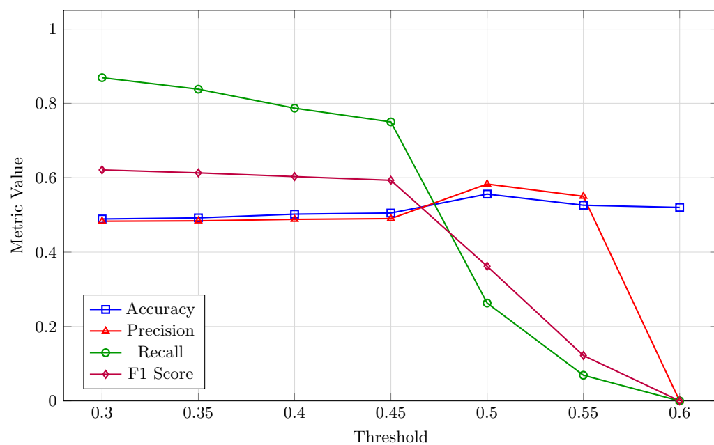
Figure 1: Threshold sweep showing Accuracy, Precision, Recall, and F1 Score across different classification thresholds.
