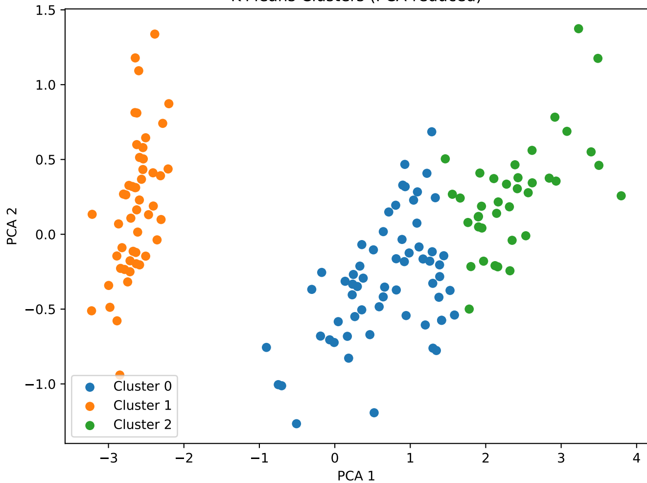
K-Means Clusters (PCA-reduced)
