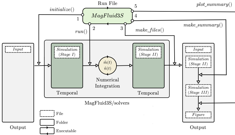
Figure 4.1. MagFluid3S workflow.
