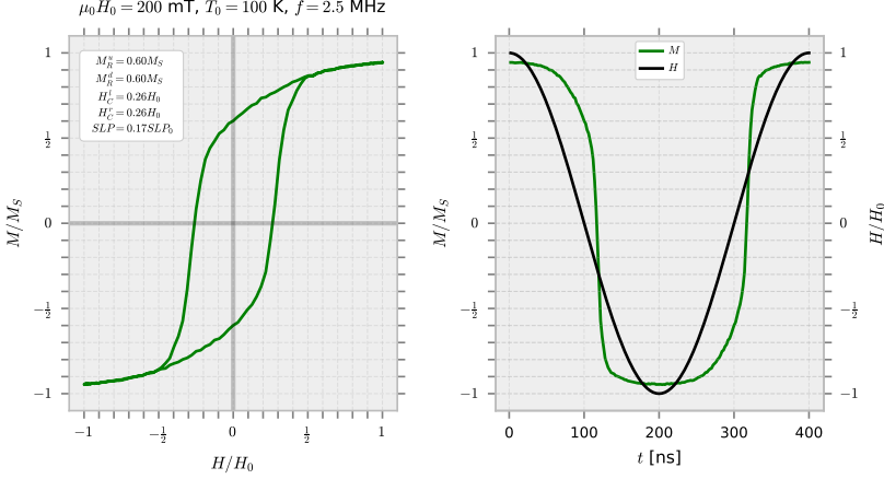
Figure 5.2. Visual output of the MvsH simulation.
