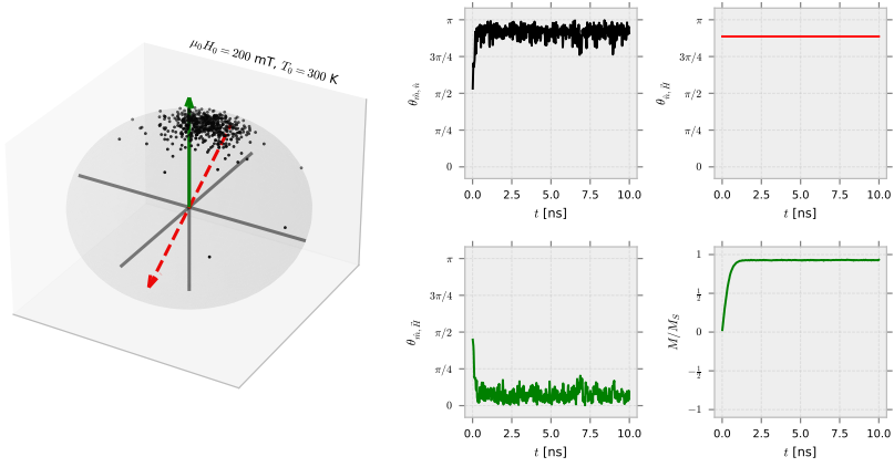
Figure 5.4. Visual output of the Microstates automation.
