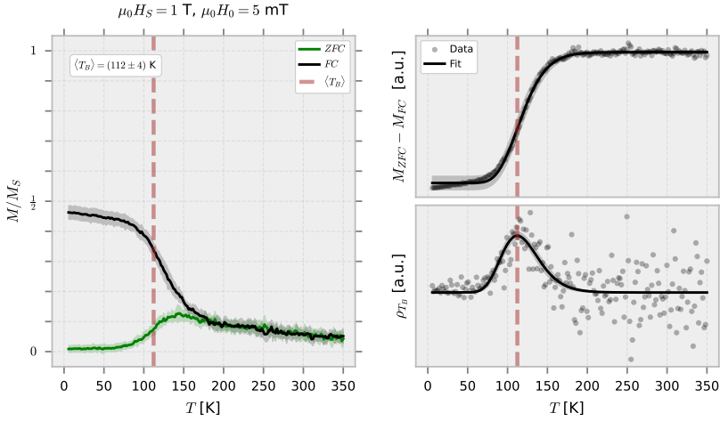
Figure 5.6. Visual output of the MvsT automation.
