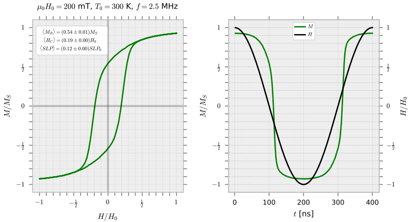
Figure 5.5. Visual output of the MvsH automation.
