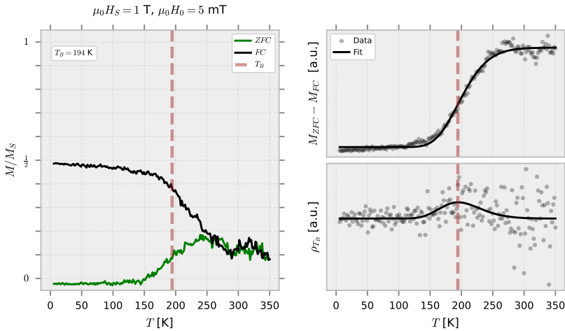
Figure 5.3. Visual output of the MvsT simulation.
