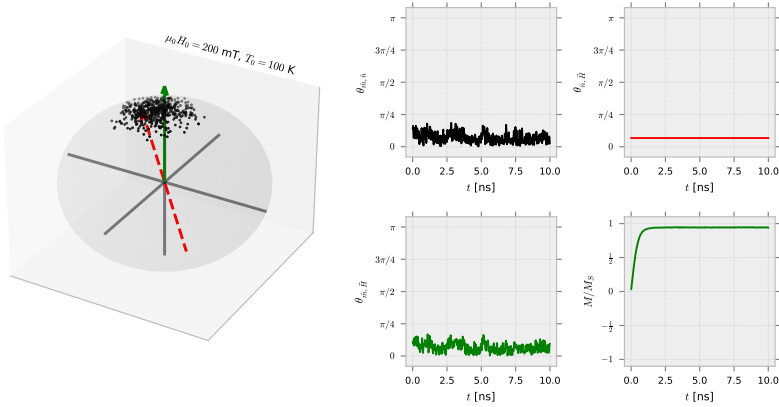
Figure 5.1. Visual output of the Microstates simulation.
