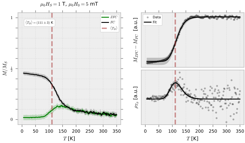
Figure 5.6. Output of the automated M vs T simulation.
