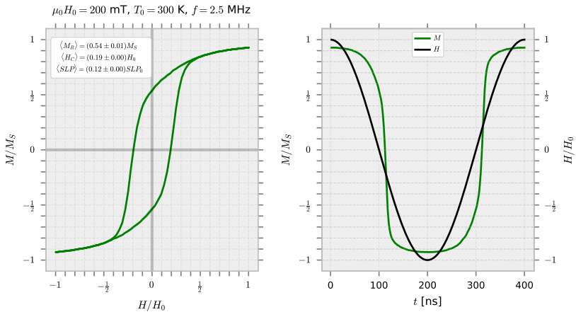
Figure 5.5. Output of the automated MvsH simulation.
