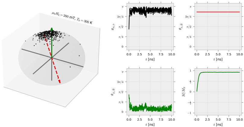
Figure 5.4. Output of the automated Microstates simulation.
