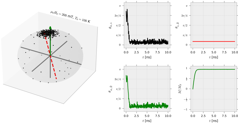
Figure 5.1. Output of the Microstates simulation.
