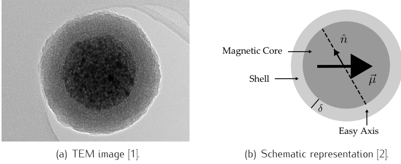
Figure 1.1. Nanoparticle structure.
