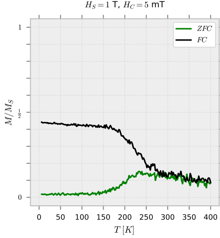
Figure 5.3. Output of the MvsT simulation.
