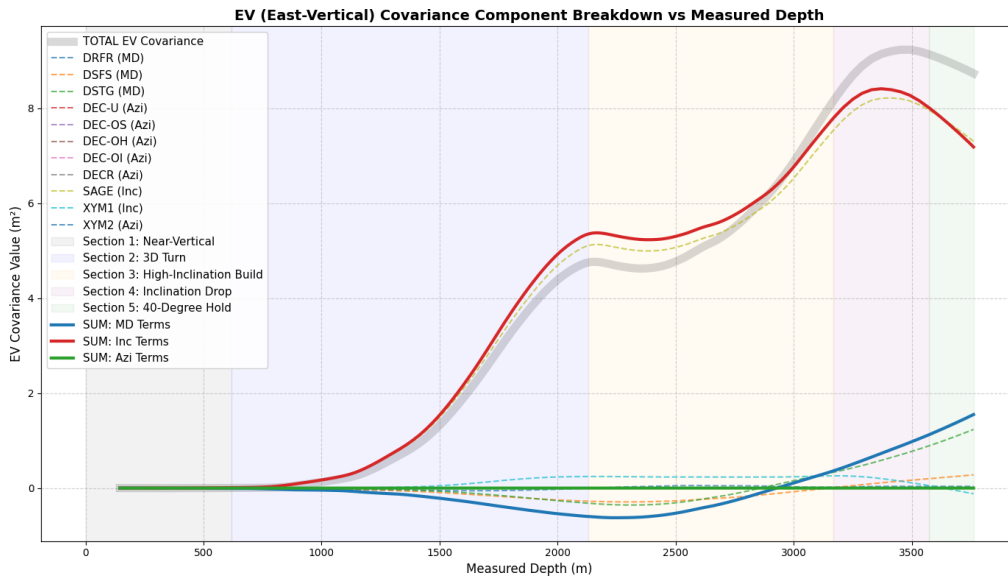
Figure 10: East–Vertical covariance contribution by error term.
