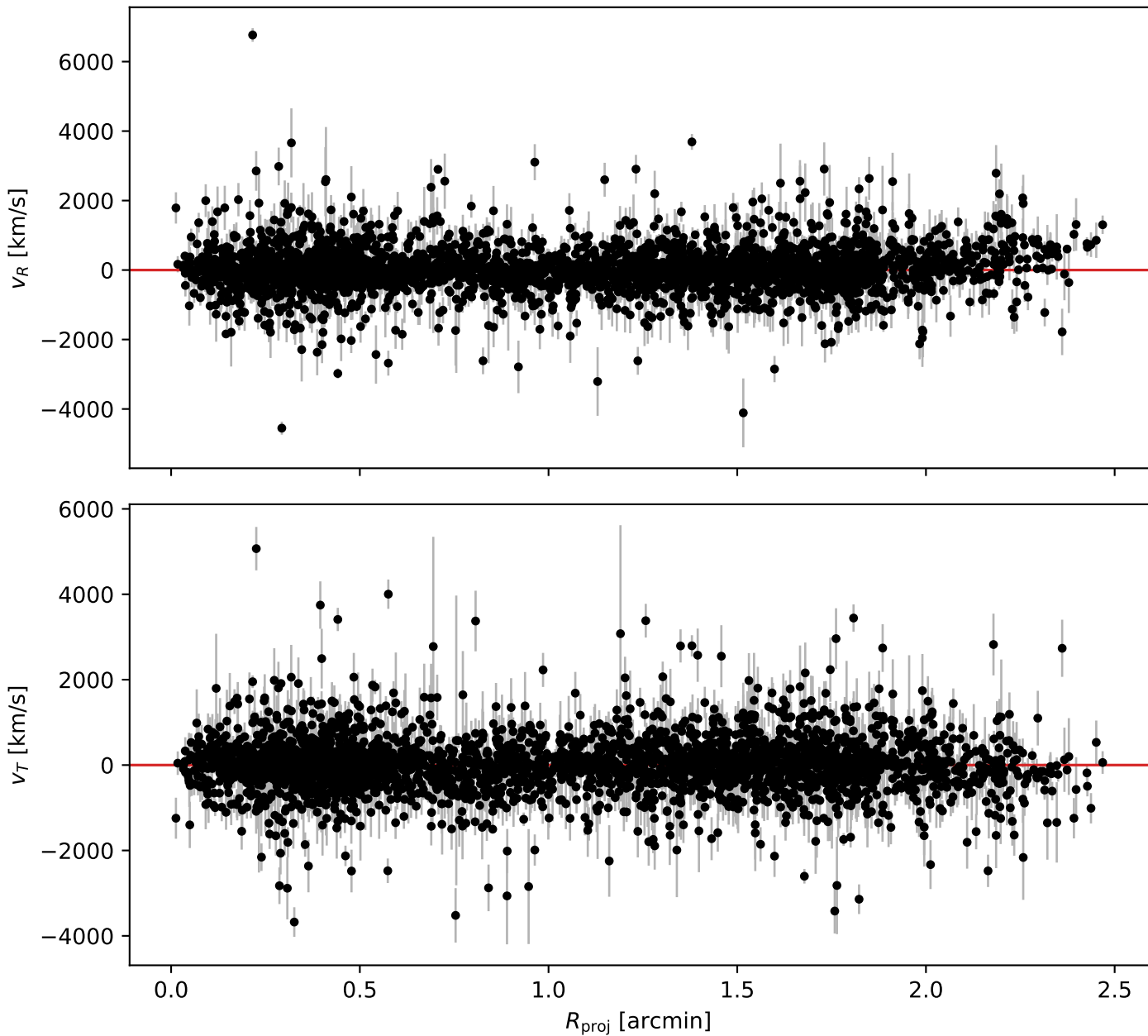
Leo II HST proper motions (bulk-subtracted)
