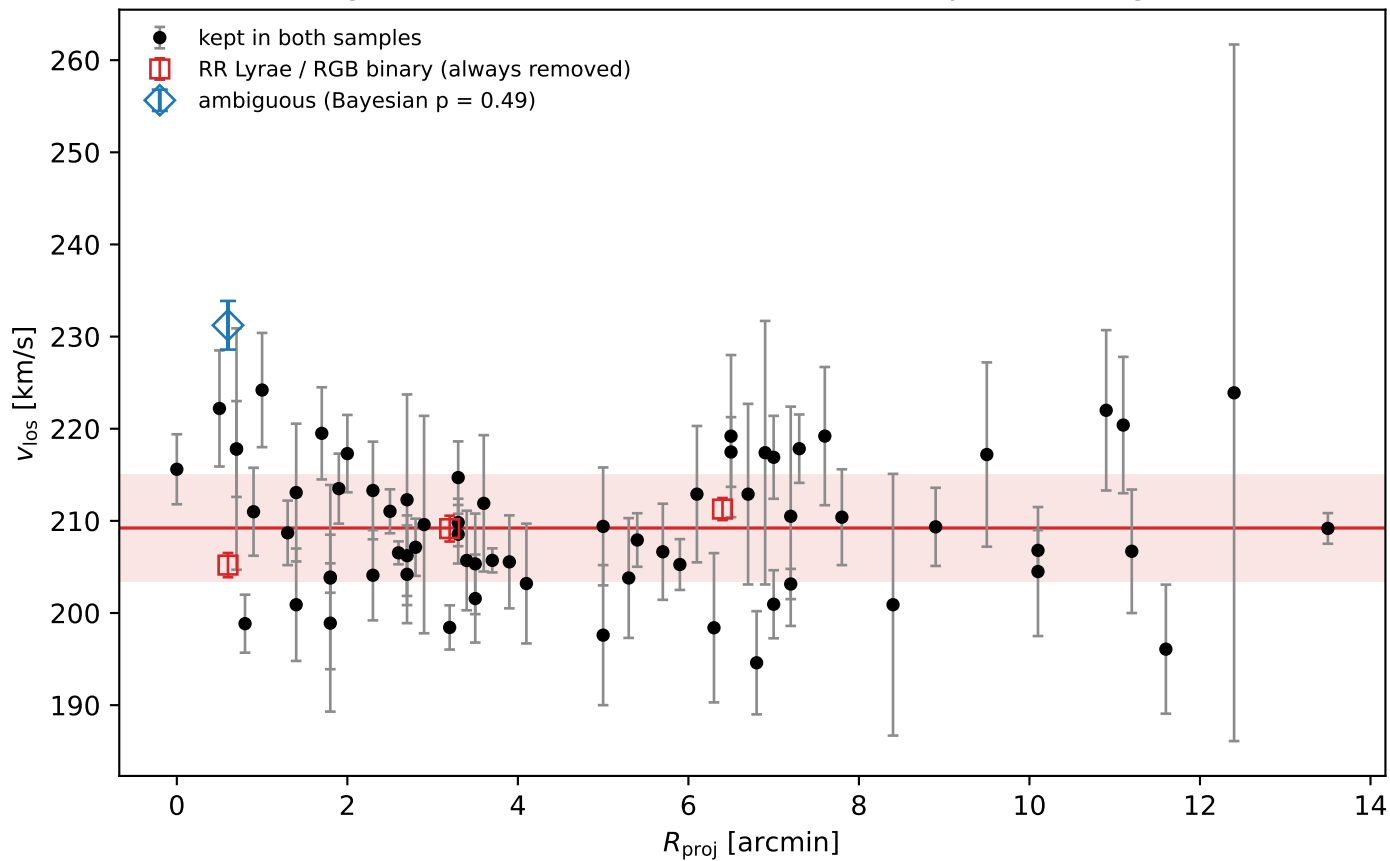
Segue 1 members (Simon+11 table 3, epoch-averaged)
