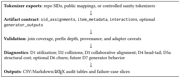
Figure 1: AUDIT-SID artifact pipeline. The current resource implements D1–D5a over item-to-SID mappings, includes optional D6 churn support, and reserves D7 for artifacts that expose generated candidates or beam traces.
