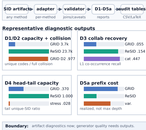
Figure 1: AUDIT-SID normalizes heterogeneous SID exports through a mapping-first contract and reports D1–D5a diagnostics. The bottom panels preview representative outputs from the Musical case study and controllers: capacity pressure, full-code collisions, collaborative-prefix recovery, head-tail allocation, and realized prefix cost. D6 is optional churn evidence; D7 requires generator outputs or beam traces.
