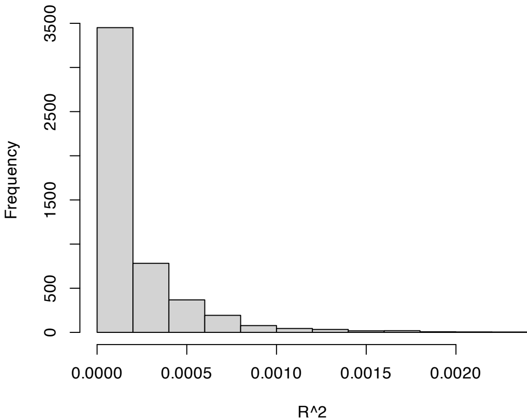
Histogram of R^2
